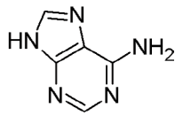
Adenine
