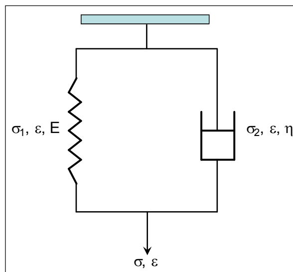
Figure 5.3 Voigt model, subjected to stress ( \sigma ) and strain ( \varepsilon )
