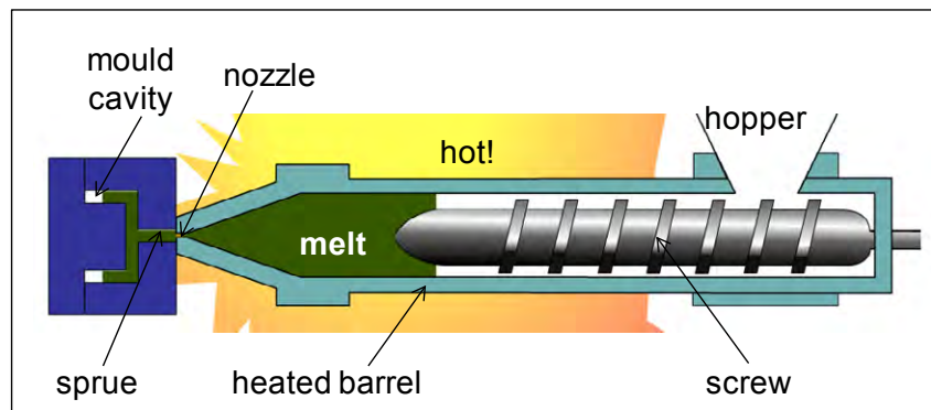
Figure 3.5 Basic elements of an injection moulding machine
