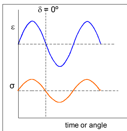
Figure 5.11 Illustration of in-phase ( \delta = 0^\circ ) oscillating stress ( \sigma ) and strain ( \epsilon ) curves
