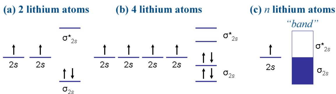
Figure 2-19: The energy levels for the molecular orbitals for lithium metal
