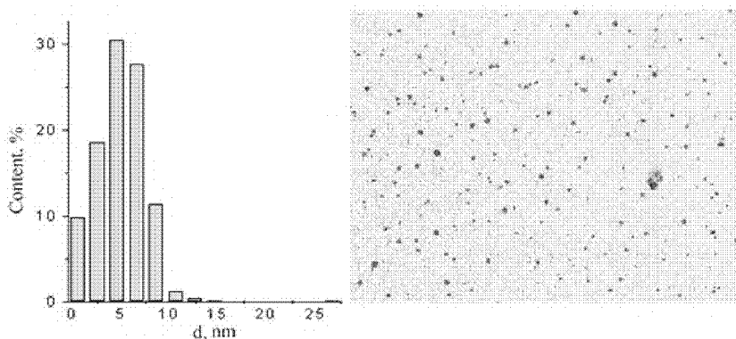
Figure 4.16 Microphotograph and size distribution of silver particles synthesized by 15-min irradiation of an aqueous solution of \text{Ag}^+\text{PA}_{1,250,000} at [\text{PA}] = 2 \times 10^{-3} \text{ M} , [\text{Ag}^+] = 6 \times 10^{-4} \text{ M} . Scale bar, -1 \text{ cm } 83 \text{ nm} .
